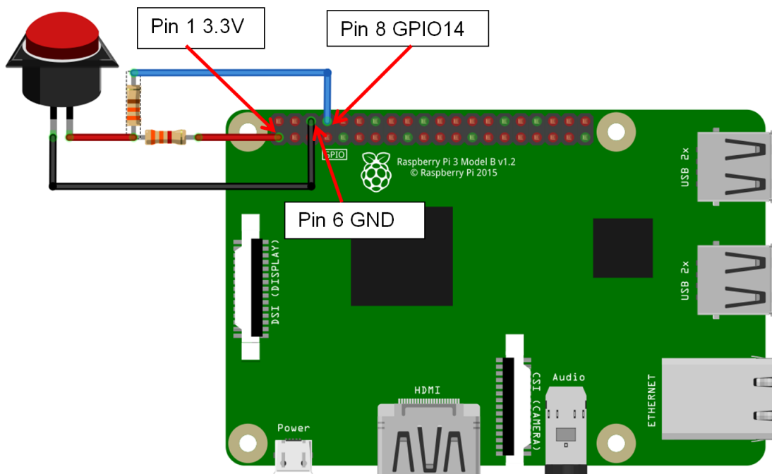
Graphical example of external Resistor pulling the GPIO 14 pin high.
